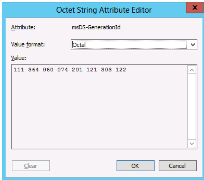
Figure 7. msDS-GenerationId Attribute
